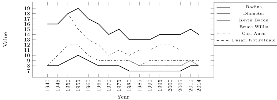
Fig. 2. Actor graph evolution in terms of radius, diameter, and actor eccentricity.
