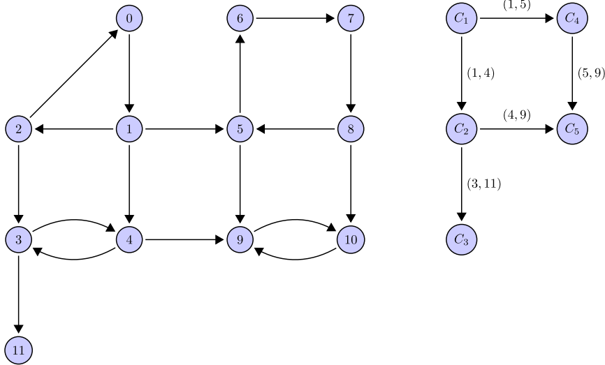
Fig. 1. A weakly connected graph and the corresponding strong component graph. Each edge (C_i, C_j) \in \mathcal{E} is labeled with a possible choice of e_{ij} .
